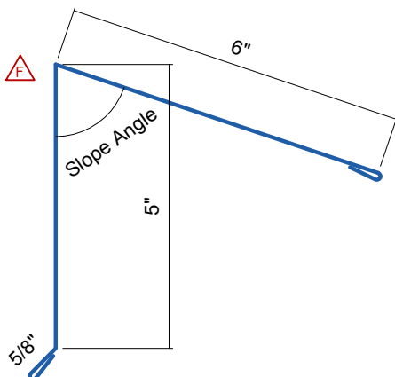
Peak Flashing
