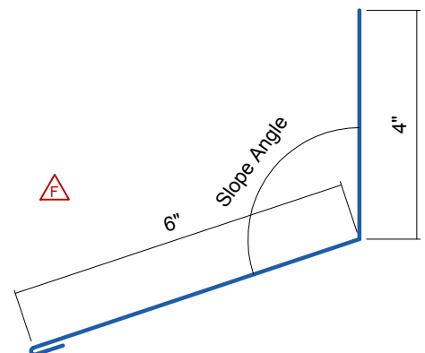
Highwall Flashing
