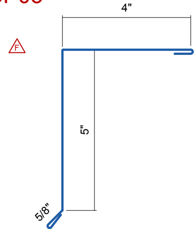
Rake Trim
